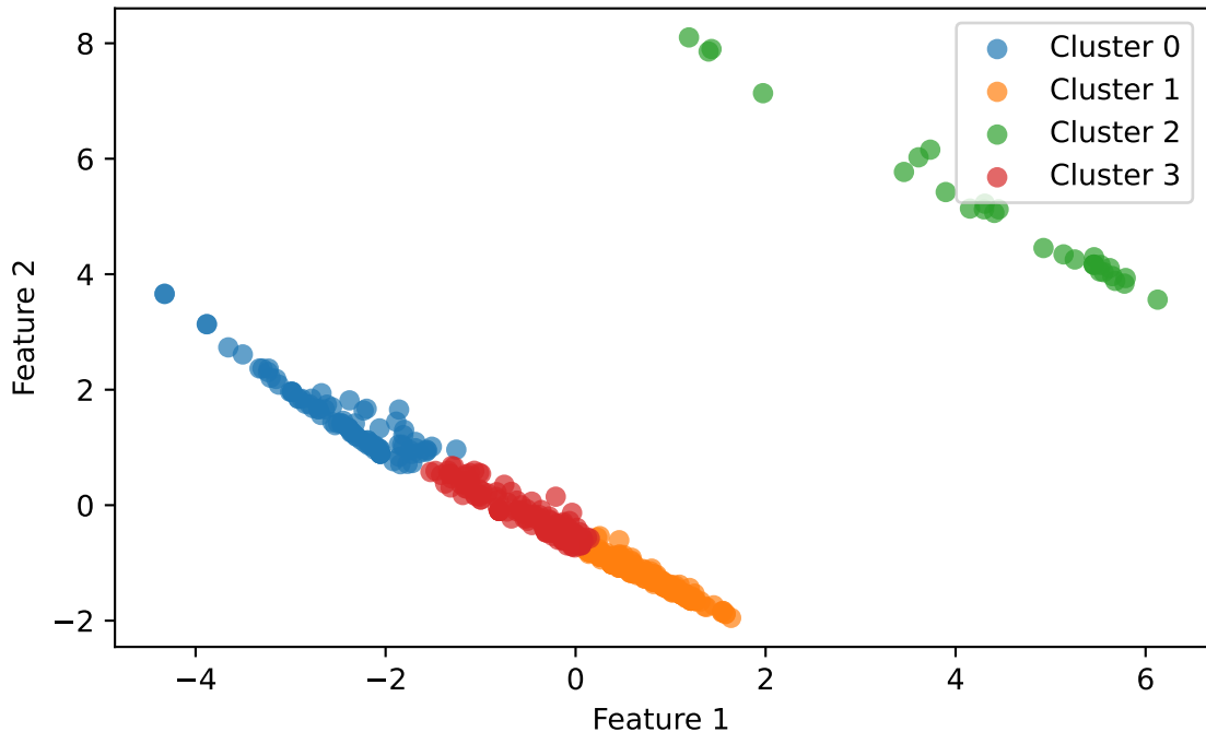
Logarithmic Standardize Data KMeans Results
