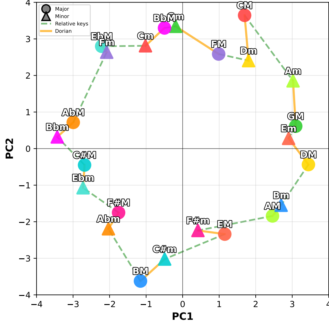
B. Piece-Level Centroids (24 pairs)
