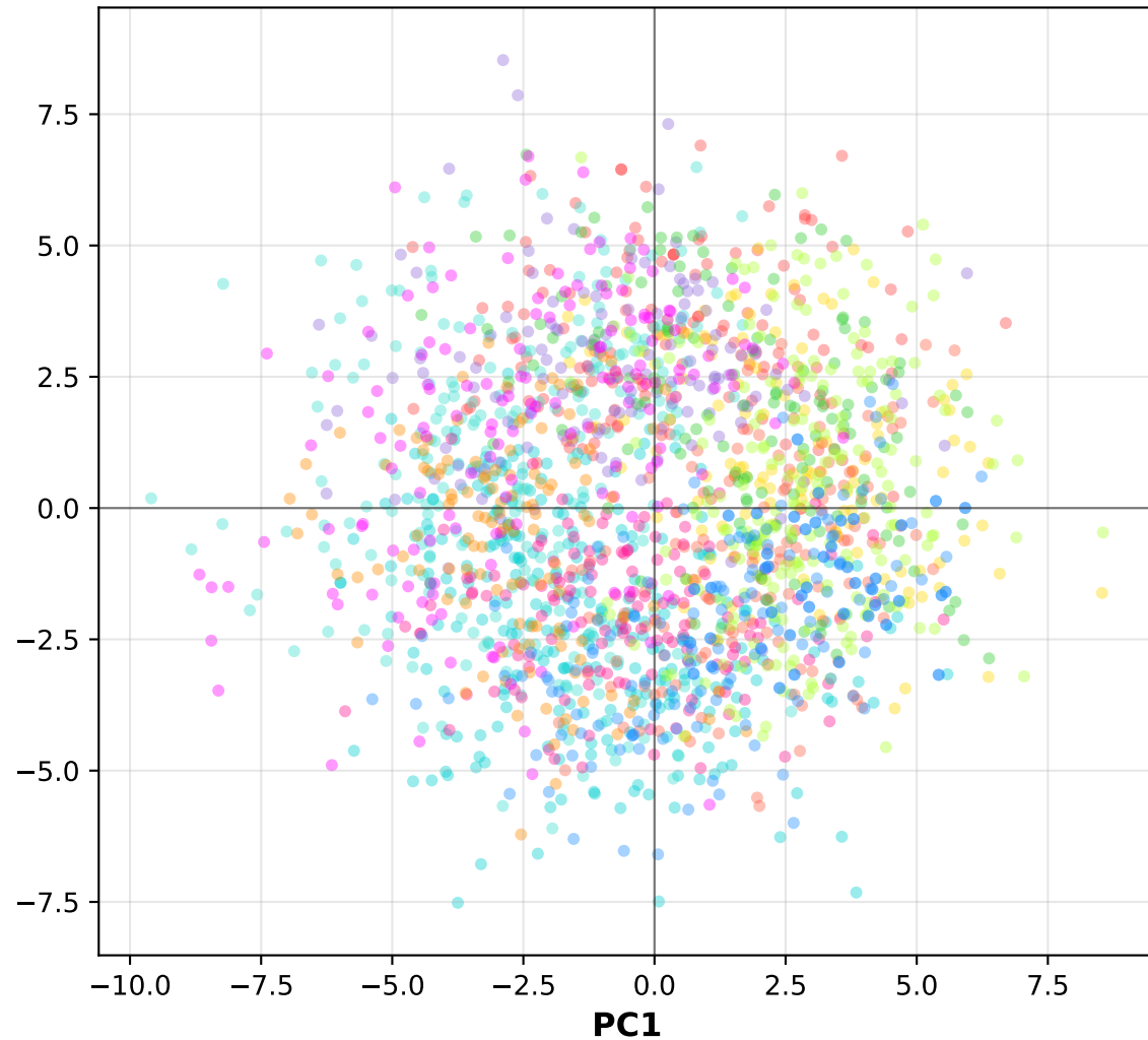
A. Individual Sequences (2,038 sequences)
