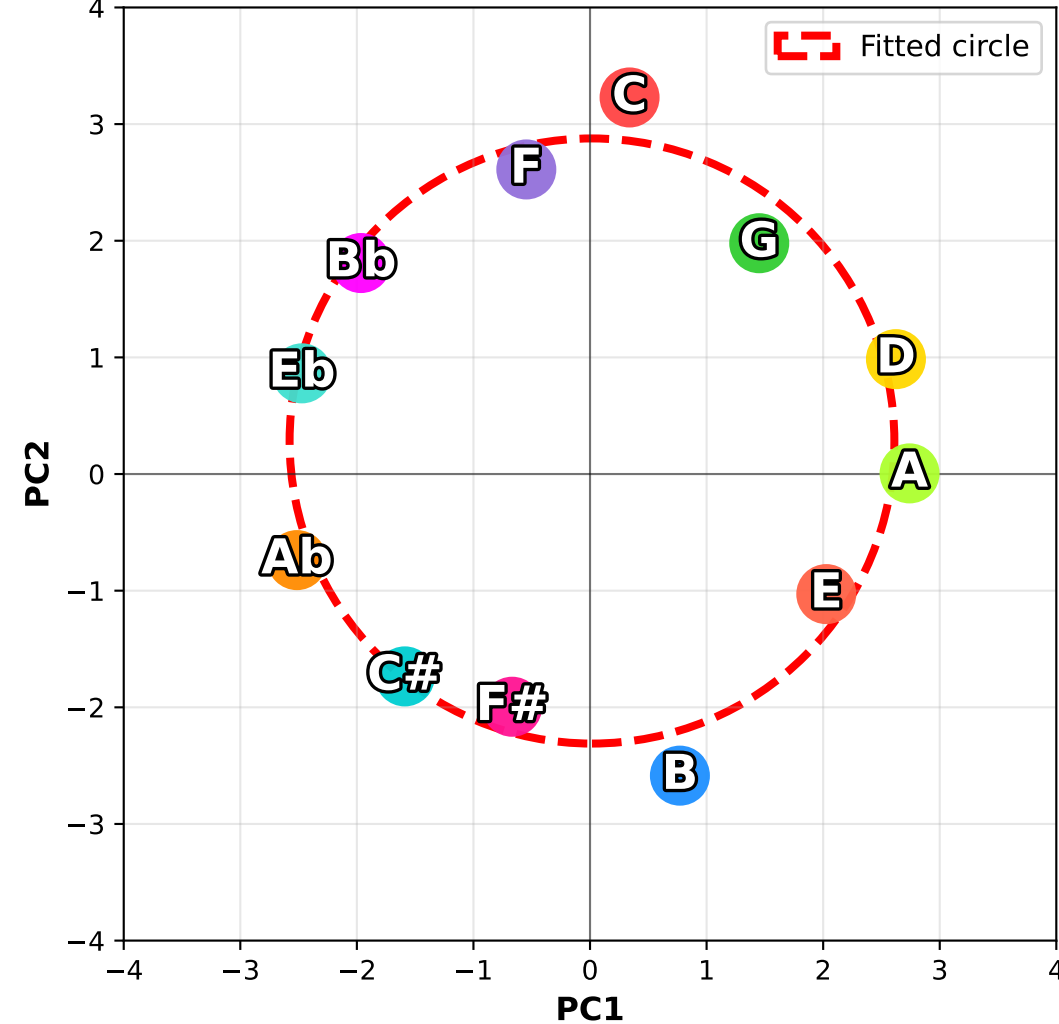
C. Circle-of-Fifths Fit (12 keys, radius=2.59 PC units)
