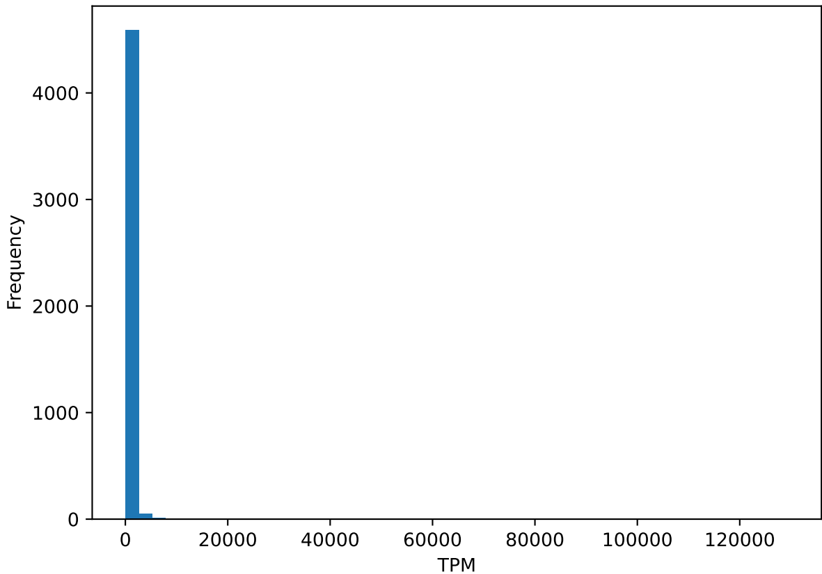
TPM Distribution
