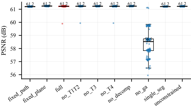
ablation at 0.1 bpp
