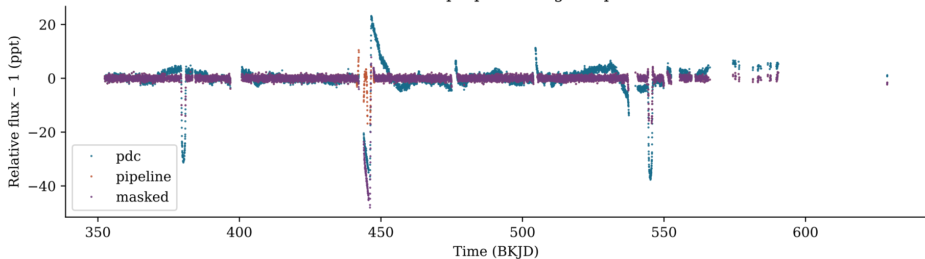
KIC 8308347: preprocessing comparison
