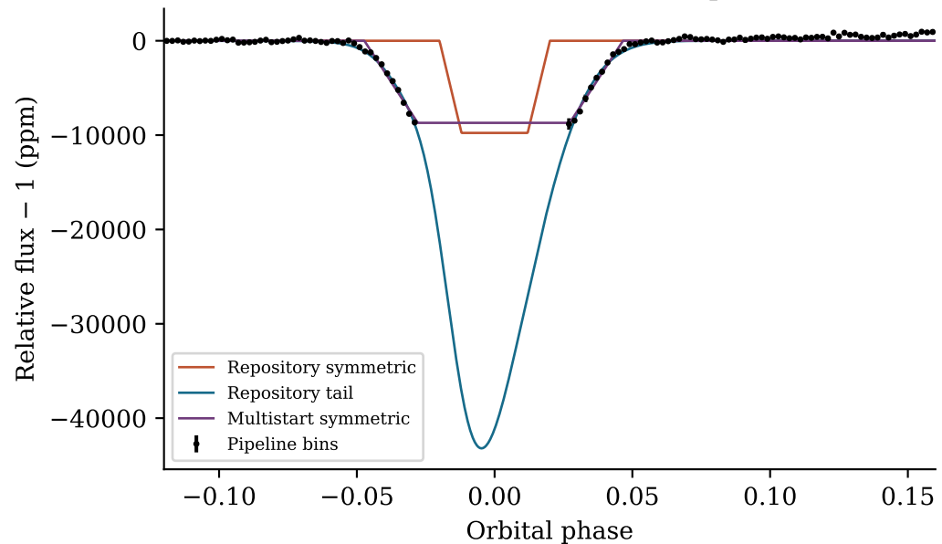
Quarter-resolved PDC-SAP
