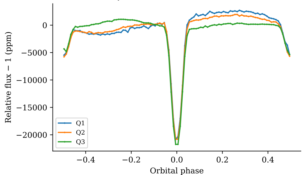
Quarter-resolved PDC-SAP
