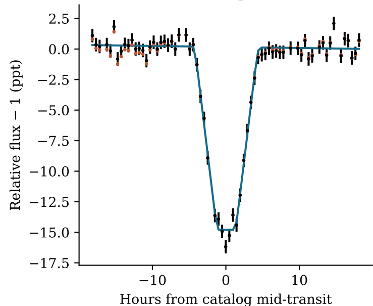
KIC 10153011, epoch 3, N=68
