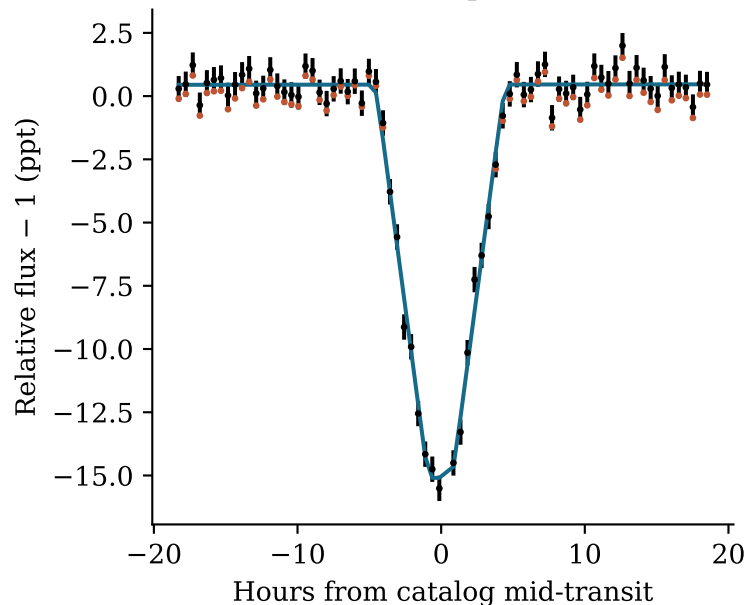
KIC 10153011, epoch 2, N=75
