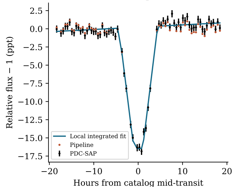
KIC 10153011, epoch 1, N=70
