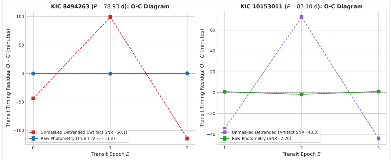
Exomoon Perturbation Signatures & TTV Analysis
