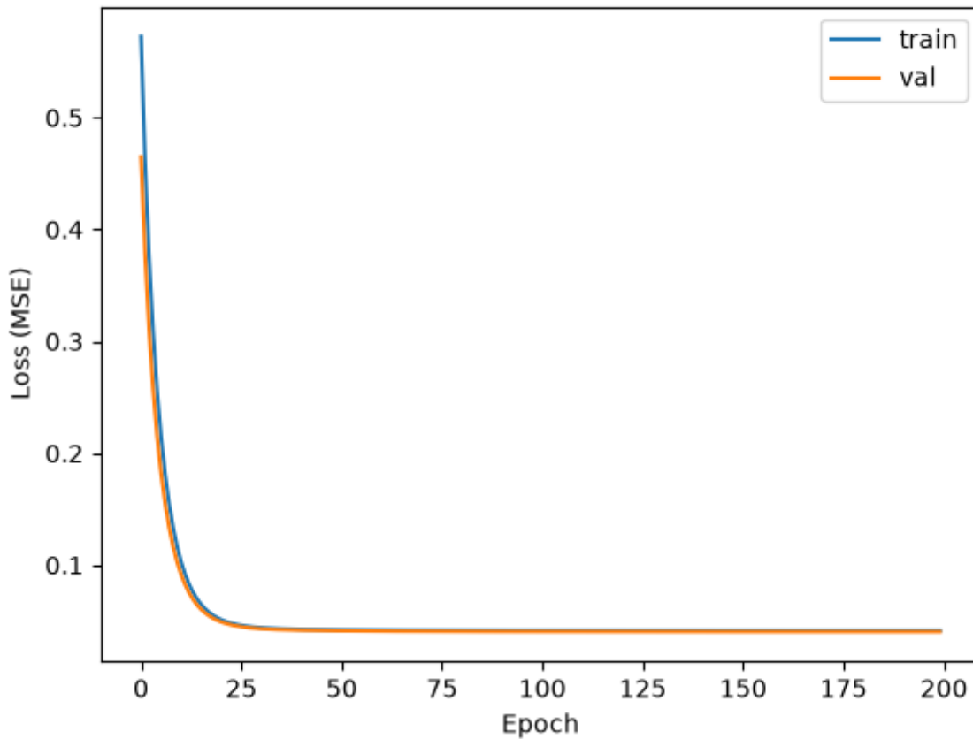
COUGHVID (real data, n=27550) - Train vs Val Loss
