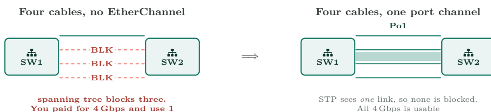
Figure 11.1: Bundling is not about speed for one conversation — it is about spanning tree seeing one link instead of four, and therefore blocking none of them.
