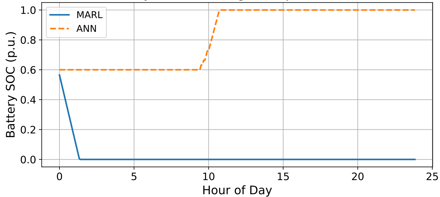
Battery State of Charge Comparison (24h)
