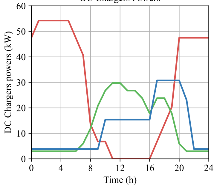
DC Chargers Powers
