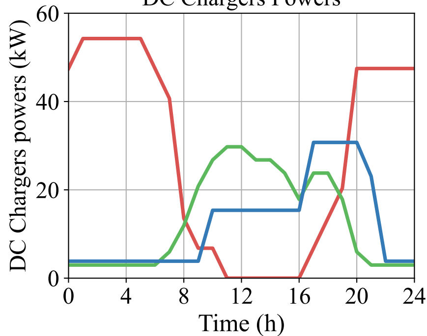
DC Chargers Powers
