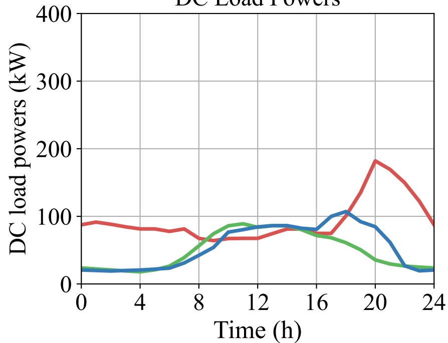
DC Load Powers
