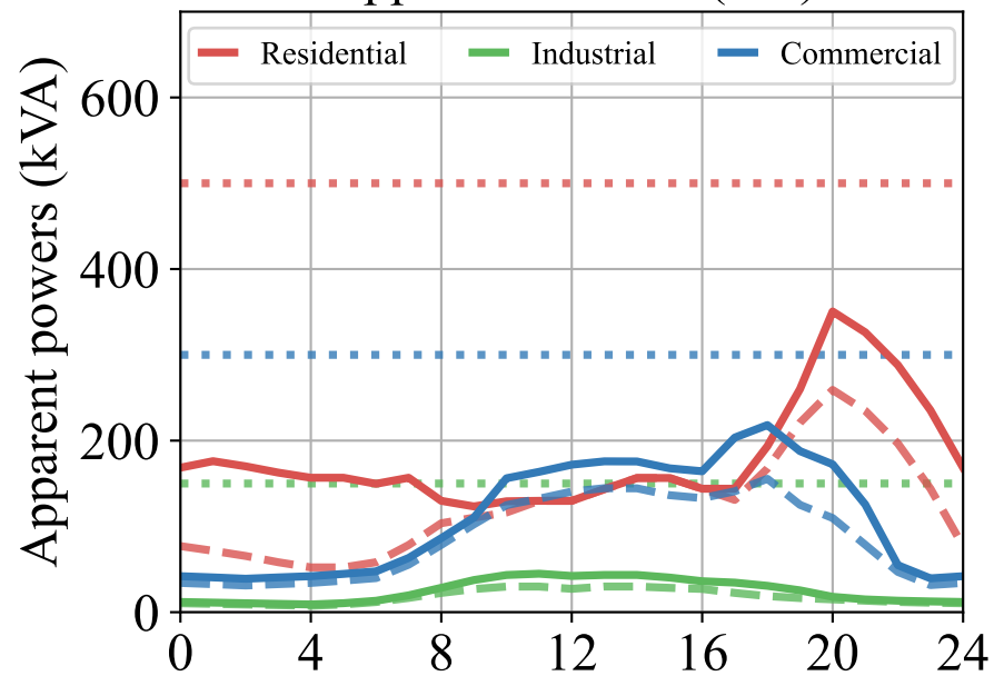
Apparent Powers (AC)
