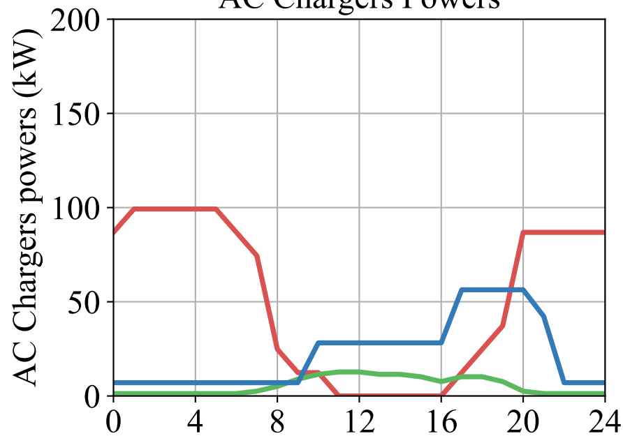
AC Chargers Powers
