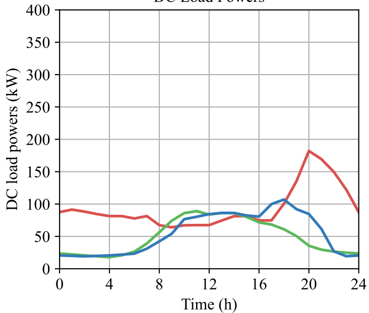
DC Load Powers
