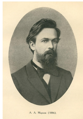
Andrei Markov
