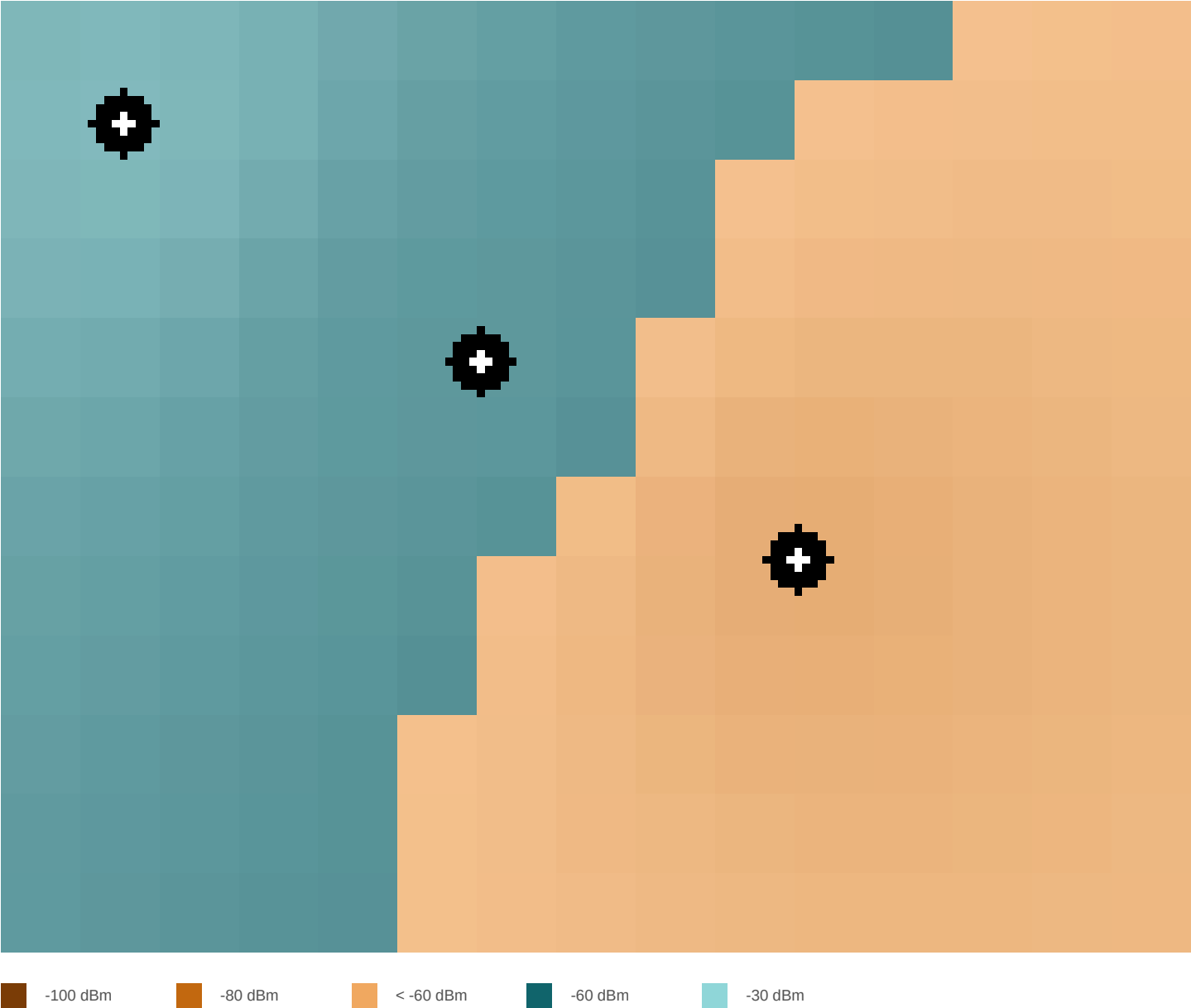
Coverage Map across 3 measured points, -69 to -45 dBm.
