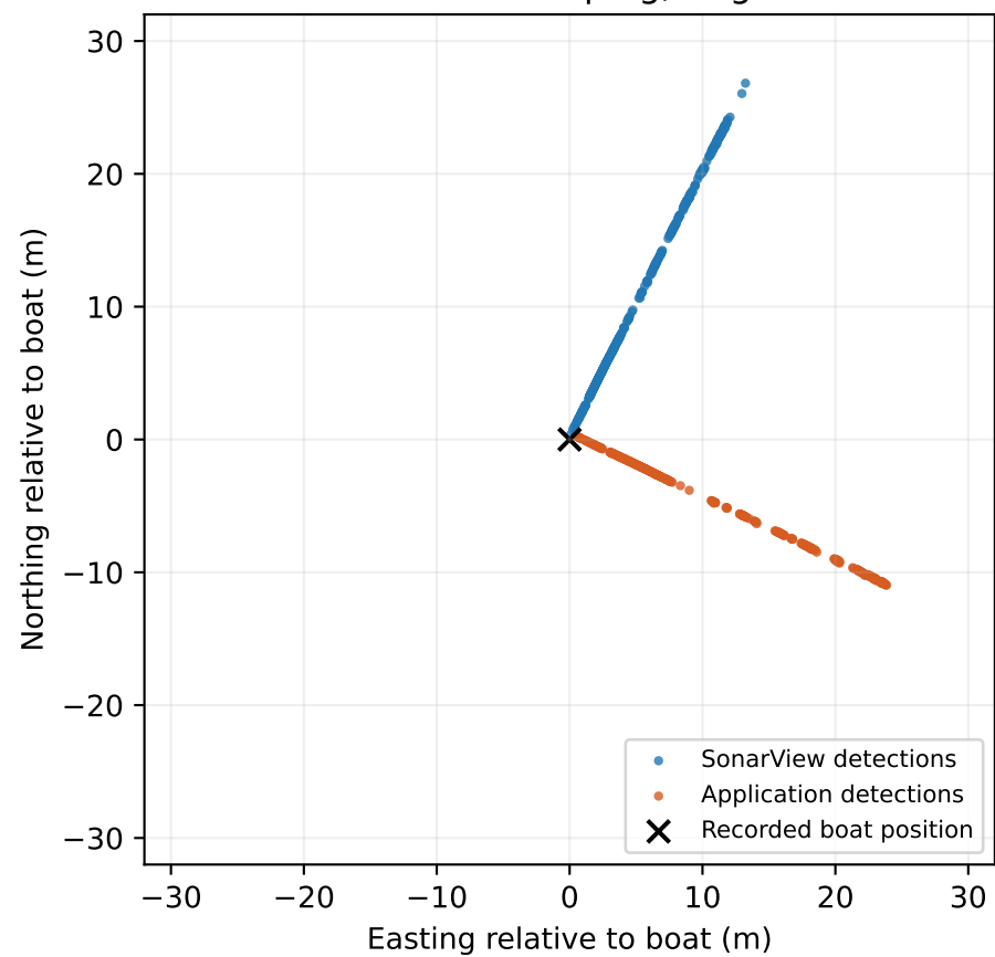
Channel 0: same recorded ping, original coordinates
