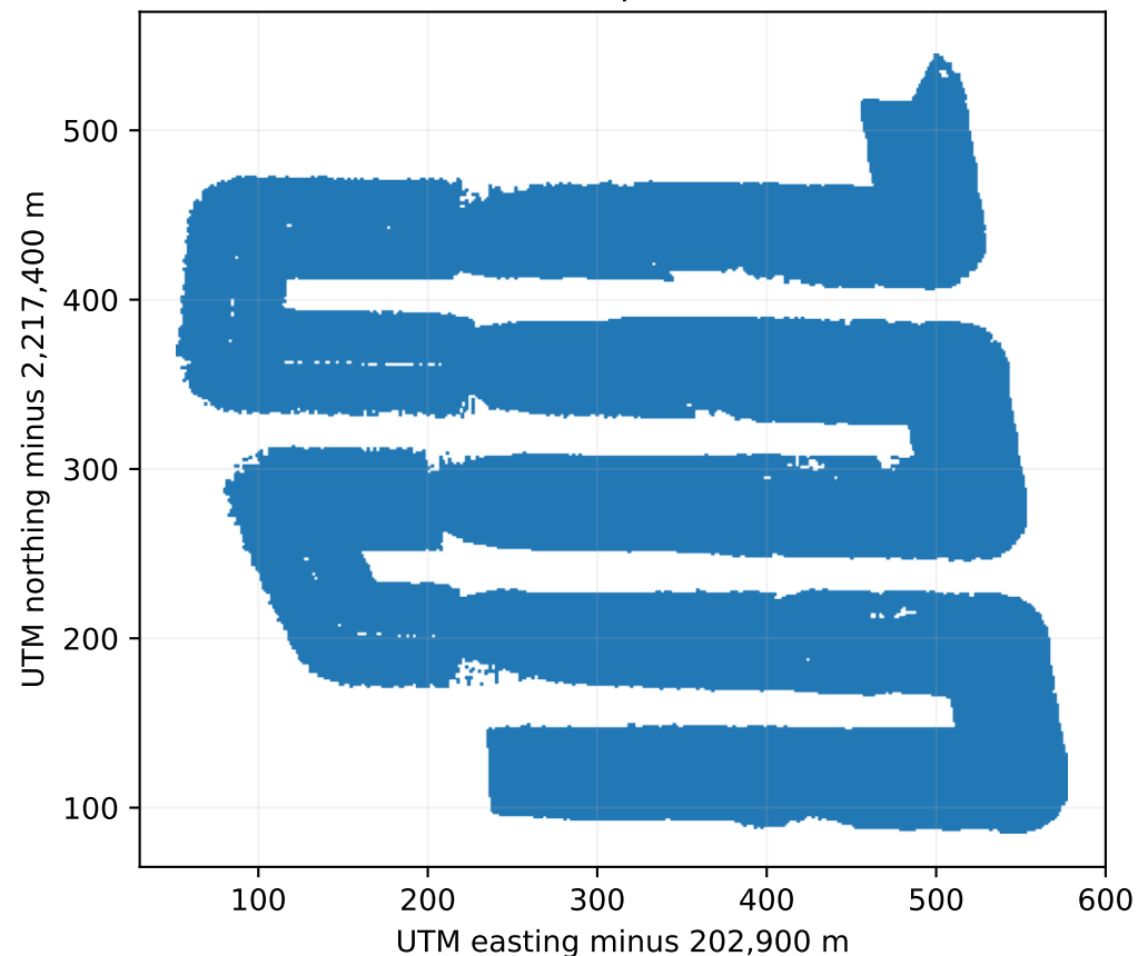
Channel 1: same recorded ping, original coordinates
