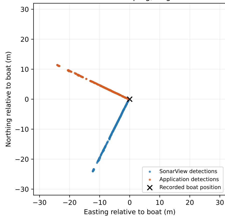
Channel 1: same recorded ping, original coordinates
