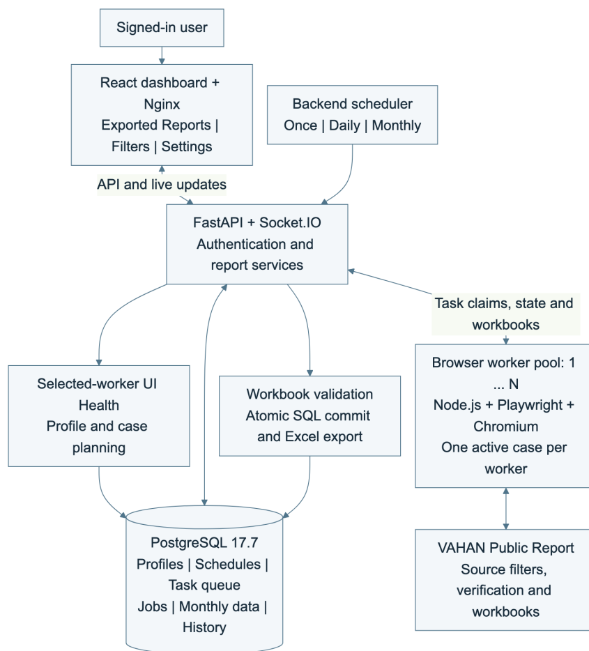
Figure 1. Current system architecture
