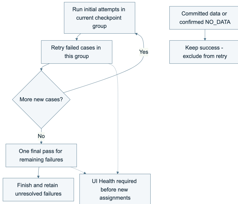
Figure 5. Checkpoint retry and final recovery
