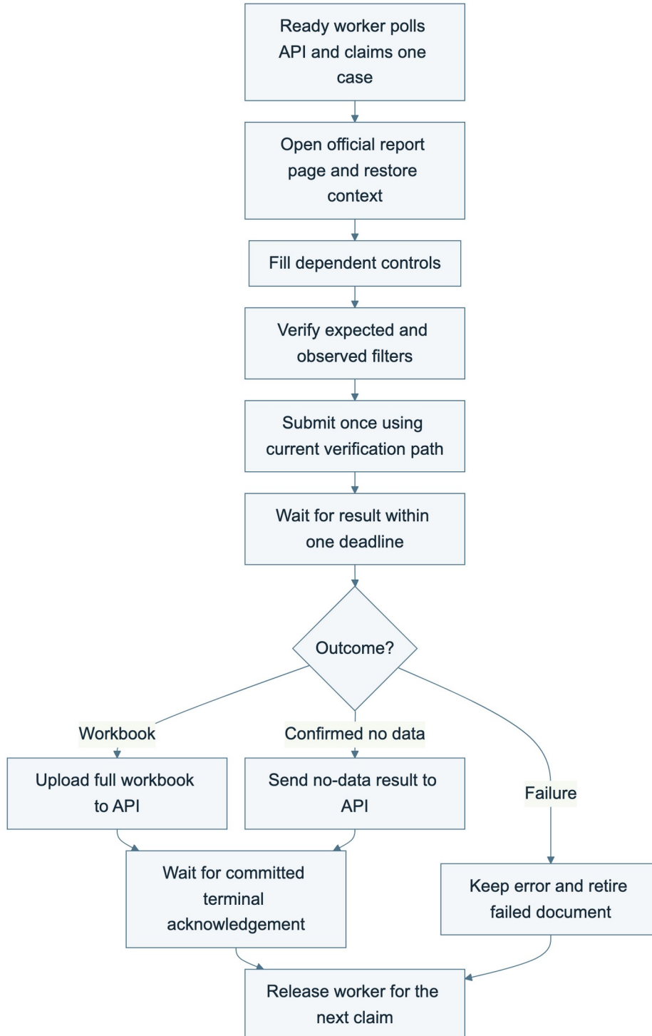
Figure 8. Crawler worker execution
