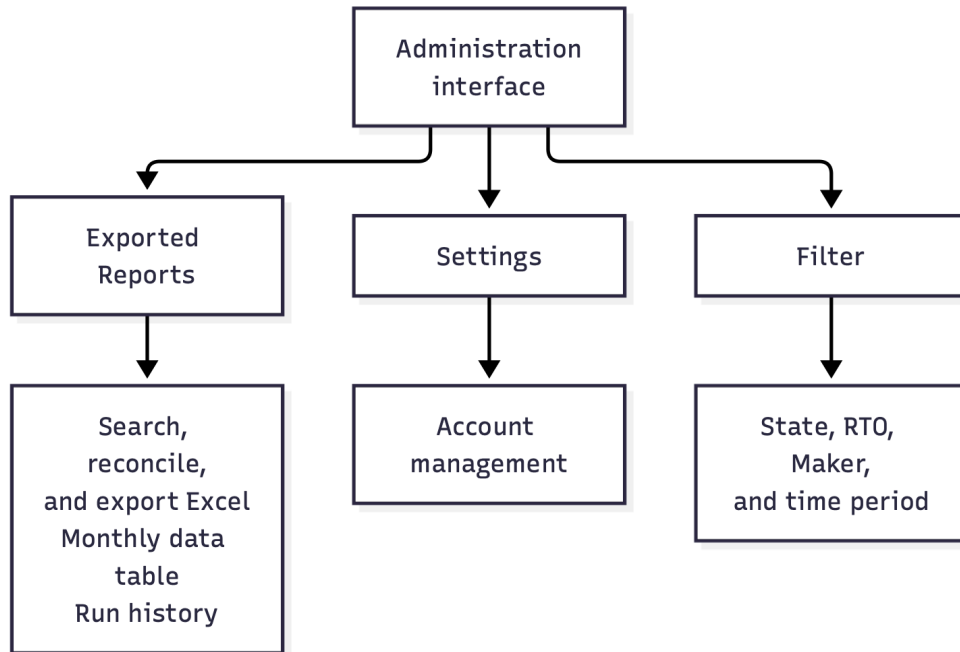
Figure 3. Functional map of the existing administration interface.
