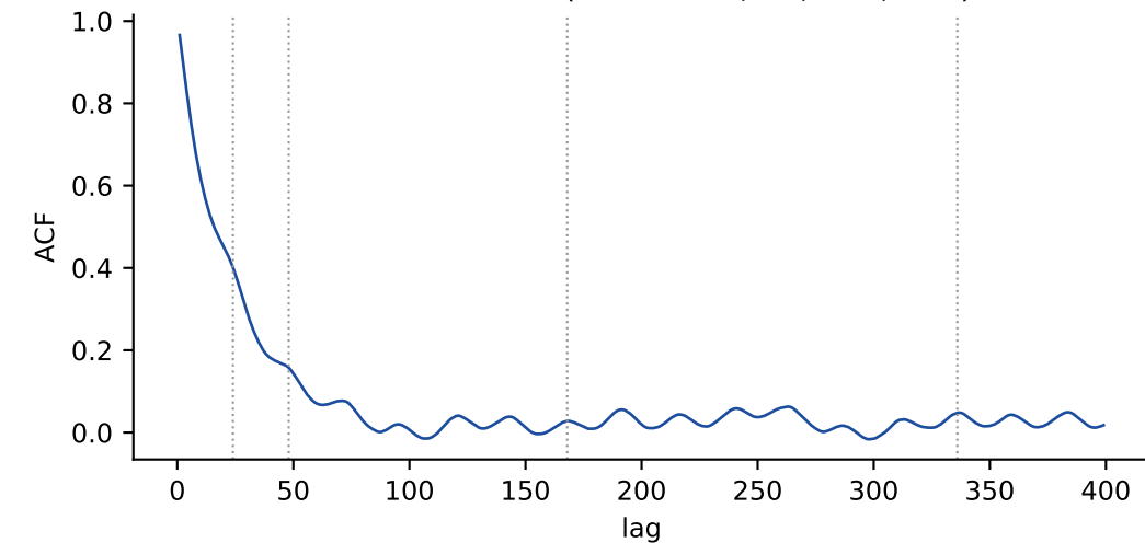
Autocorrelation (dotted: 24, 48, 168, 336)
