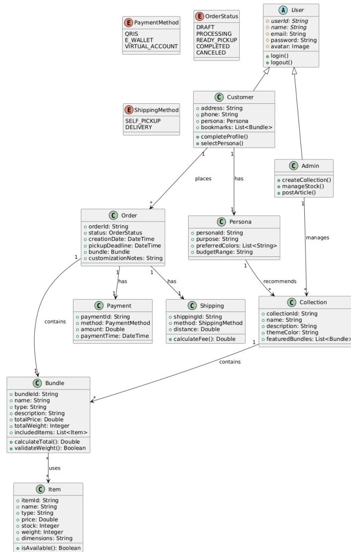
Gambar 11. Class Diagram
