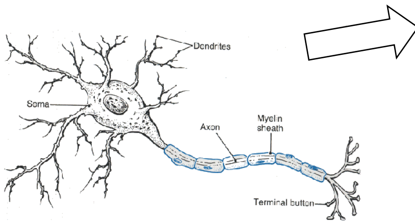
Biological neuron
