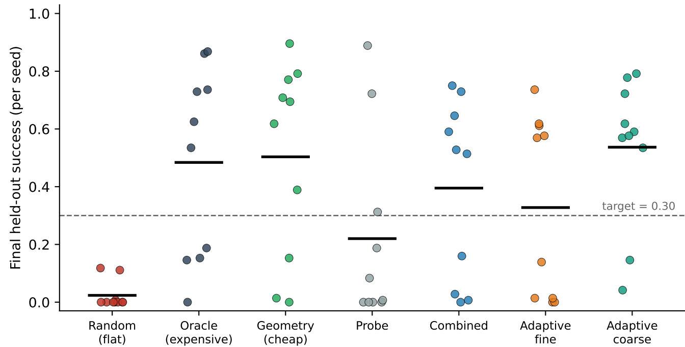
Per-seed robustness: each dot is one of 10 seeds (bar = mean)
