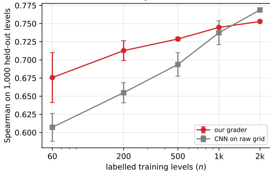
(b) Labels needed: grader vs. CNN (Sokoban)
