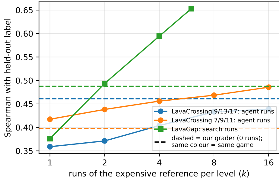
(a) A free prediction vs. running the reference k times
