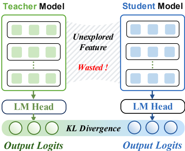
(a) Vanilla OPD
