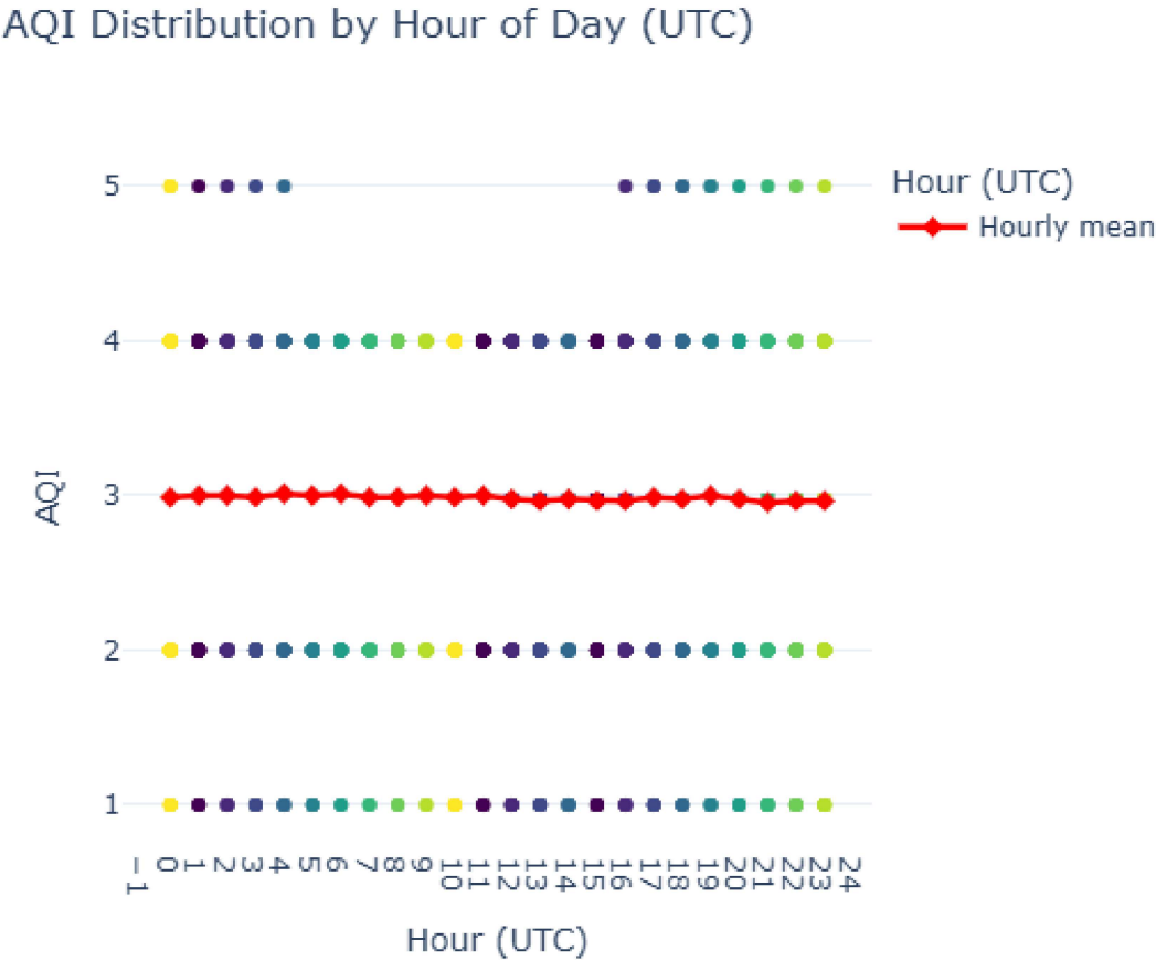
Figure 4: Hourly Pollution Pattern (Diurnal Cycle)
