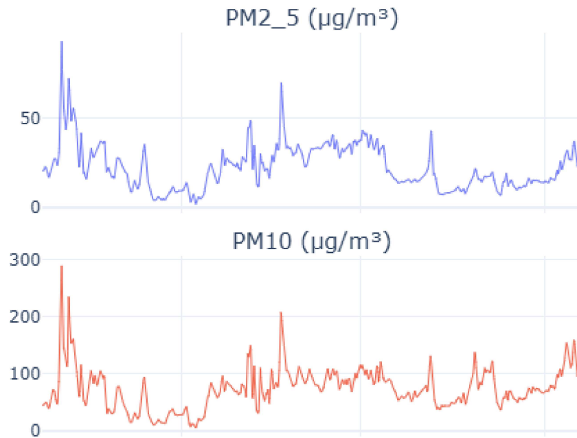
Figure 2: PM2.5 PM10 Trend Over Time
