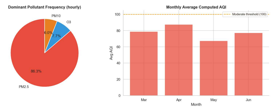
Figure 7: Pollutant / EPA AQI Distribution
