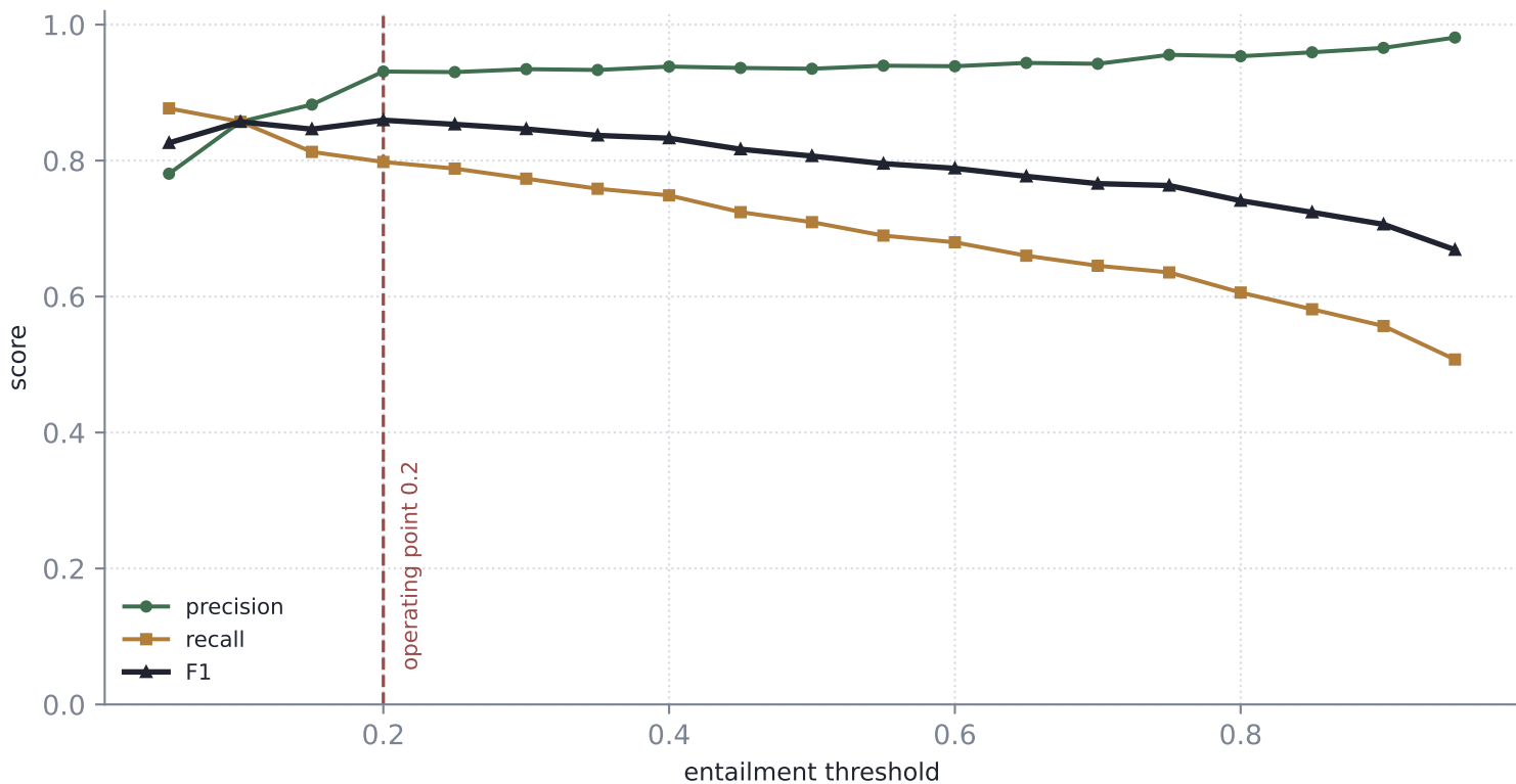
Module D threshold calibration (600-pair labeled slice)
