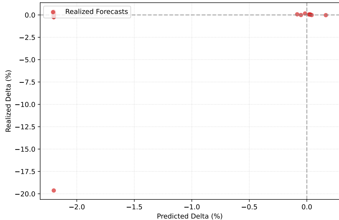
Predicted vs Realized Return % (MAE: $1,798.58)
