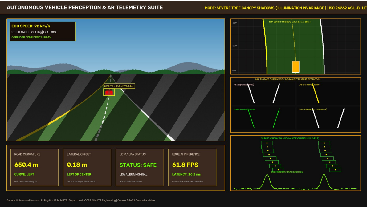
Figure 4: Executive Vision Telemetry Dashboard Under Challenging Tree Canopy Shadows (Illumination-Invariant HLS/LAB Segmentation).
