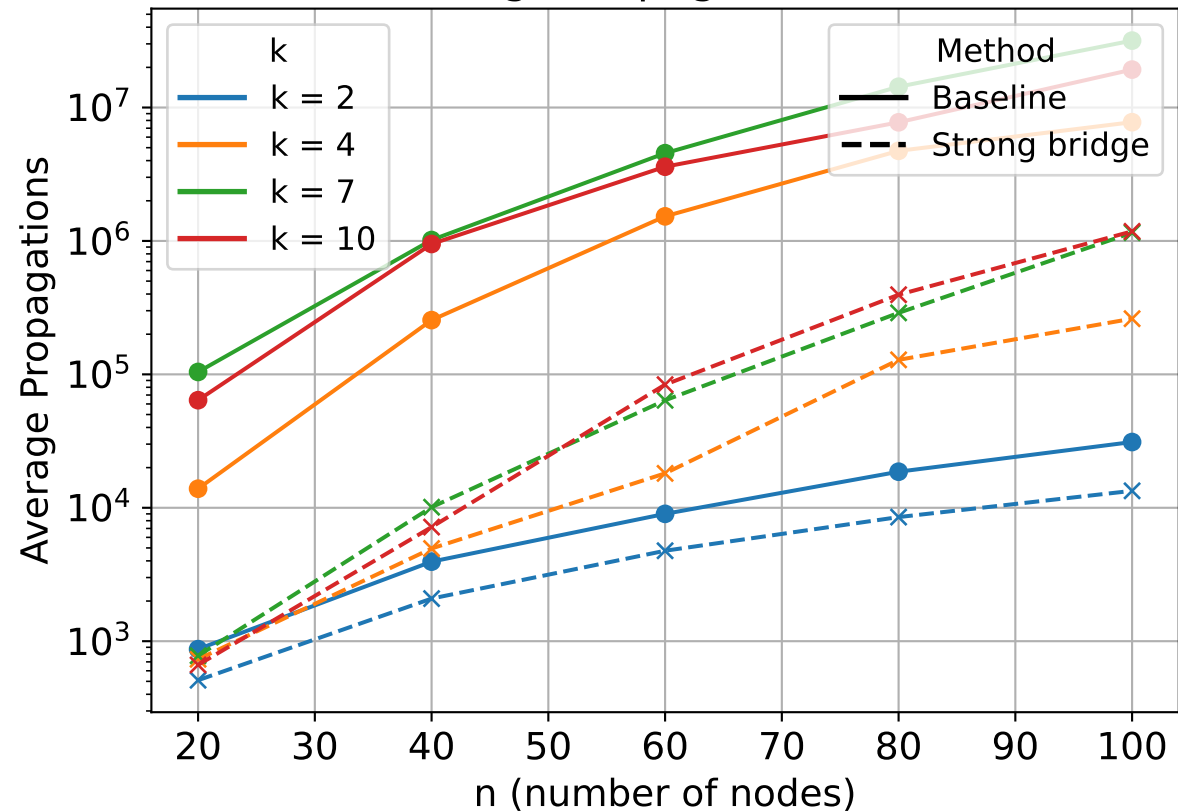
Average Propagations vs n
