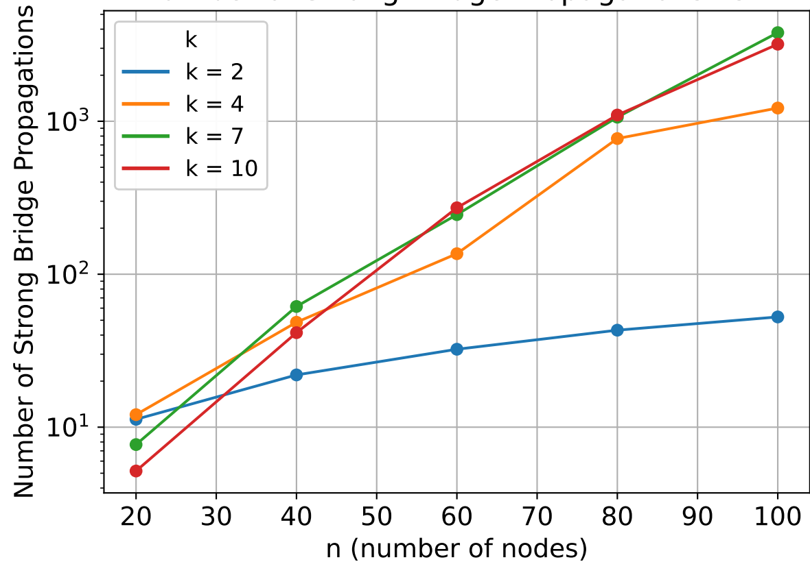
Number of Strong Bridge Propagations vs n
