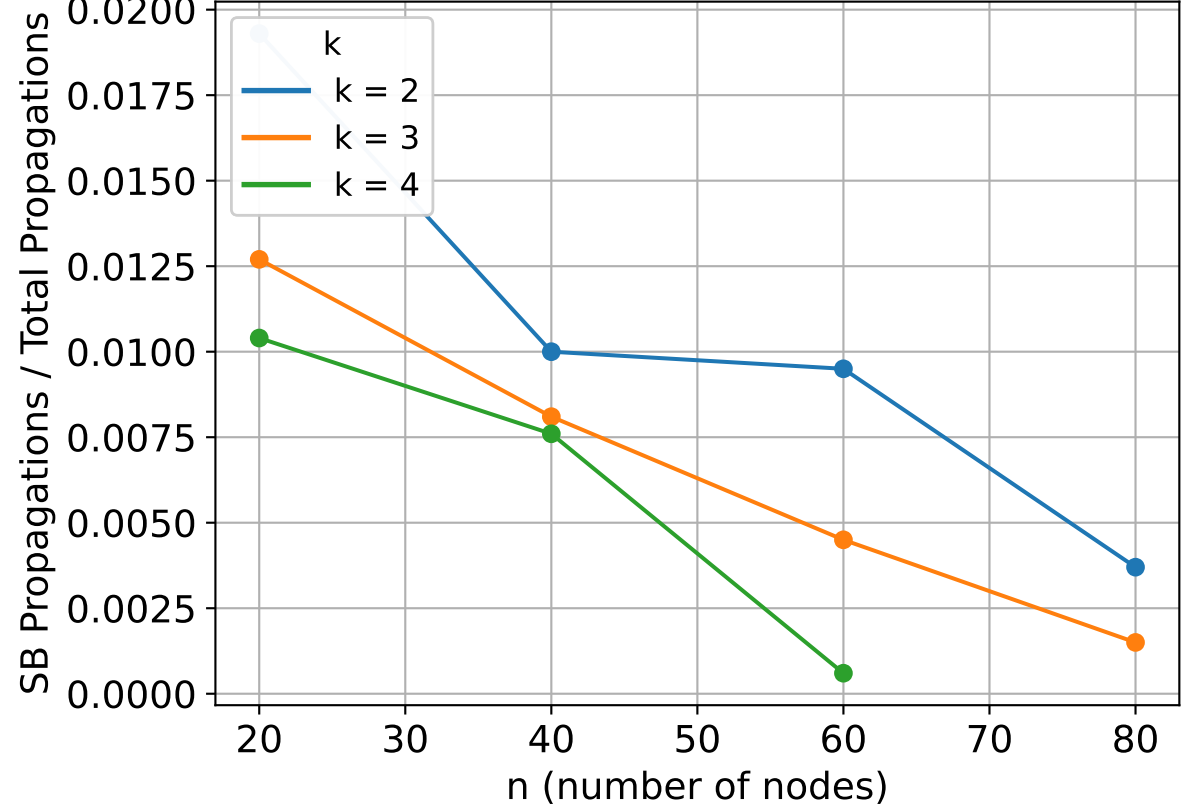
SB Propagations / Total Propagations vs Graph Size
