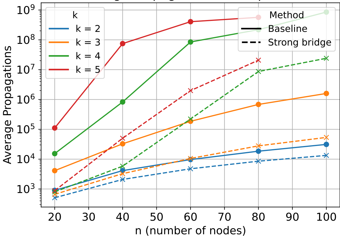
Average Propagations vs Graph Size
