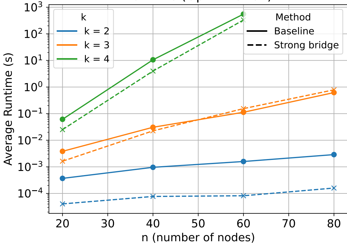
Runtime (Optimization)
