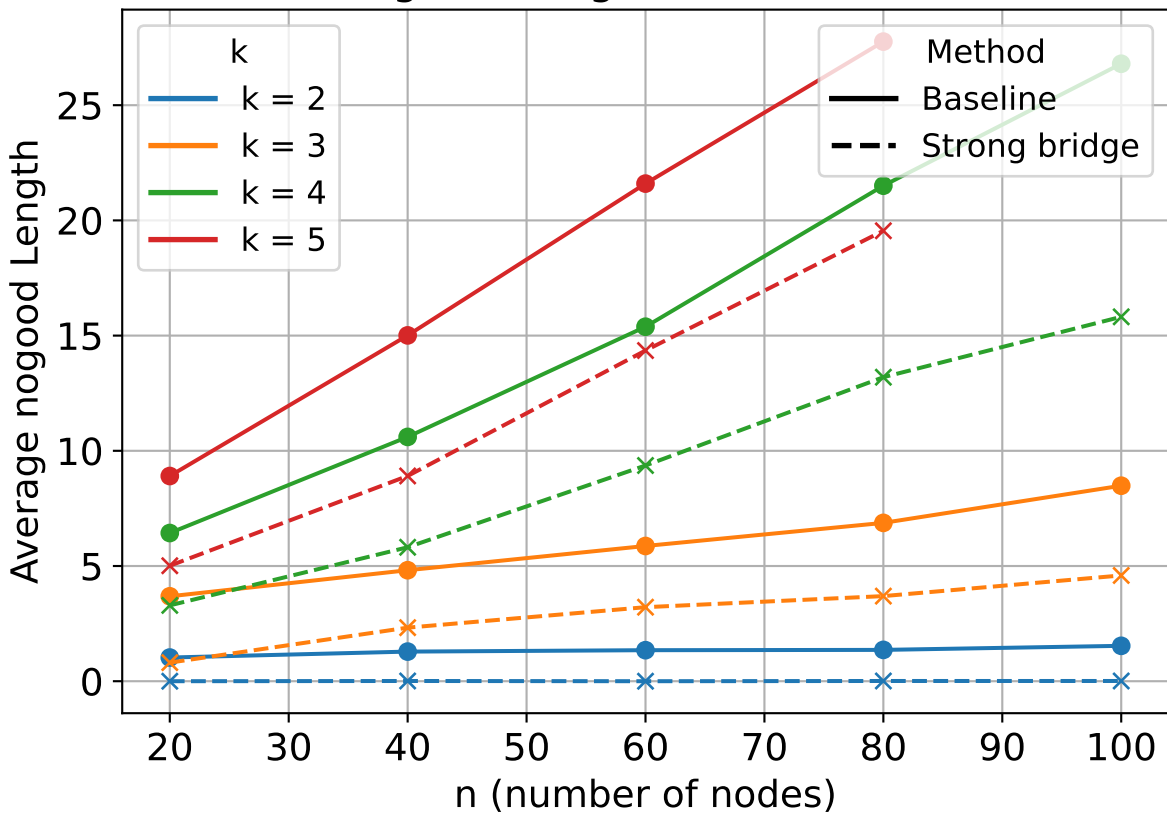
Nogood Length (Satisfaction)
