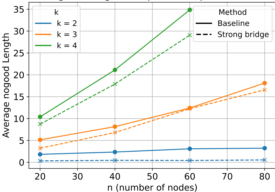
Nogood Length Comparison (Optimization)
