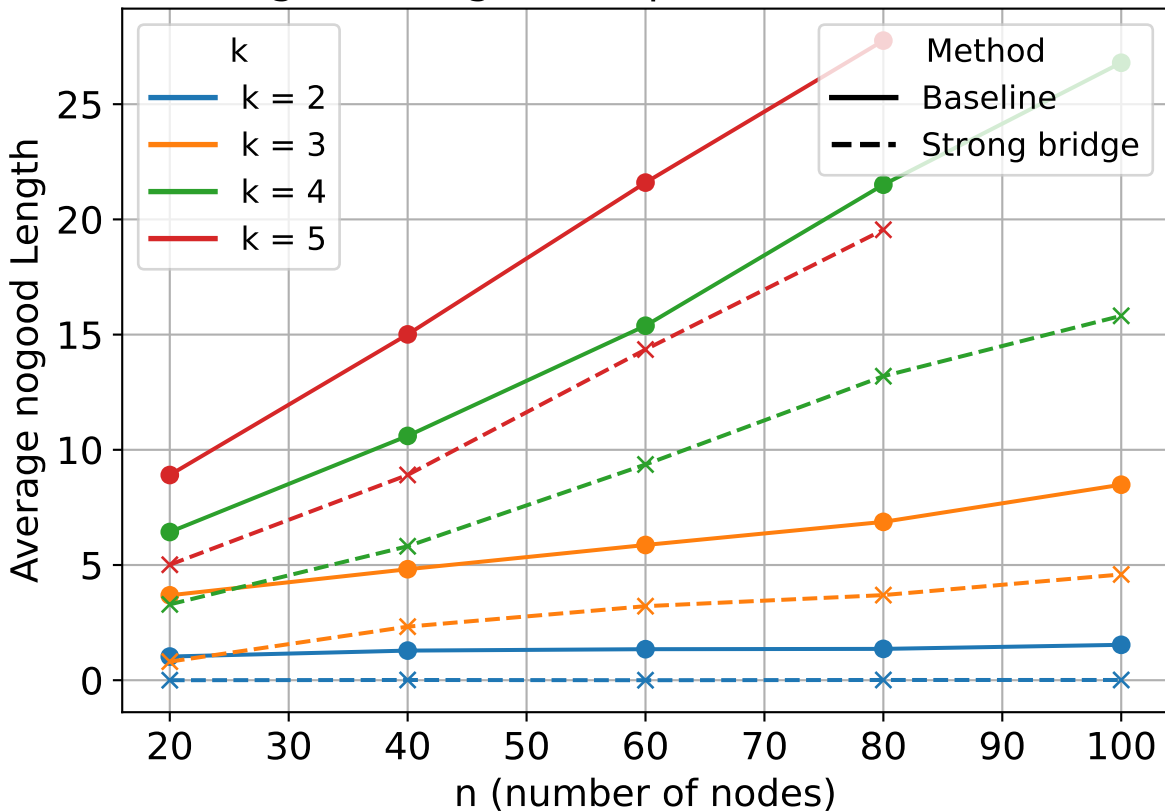
Nogood Length Comparison (Satisfaction)
