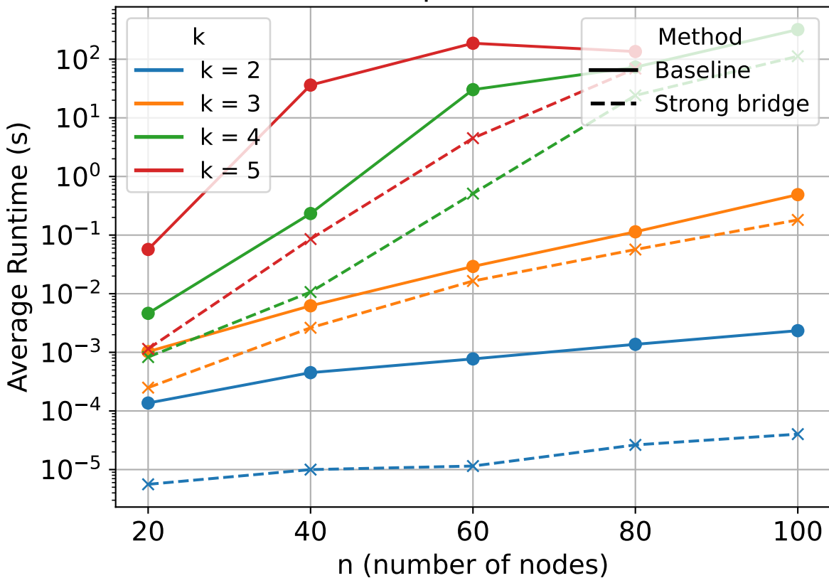
Runtime Comparison (Satisfaction)
