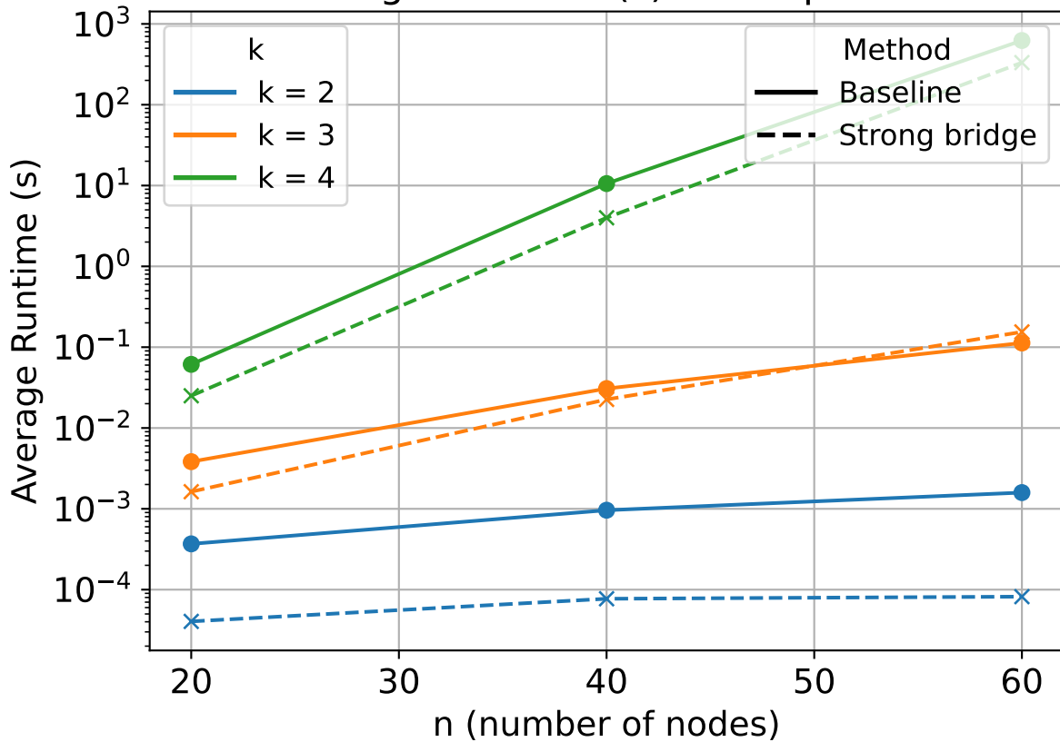
Average Runtime (s) vs Graph Size
