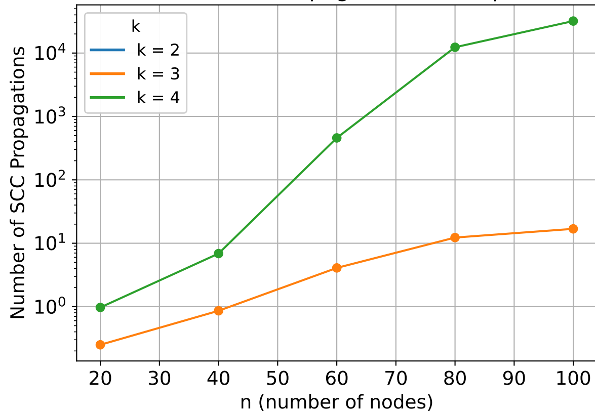
Number of SCC Propagations vs Graph Size
