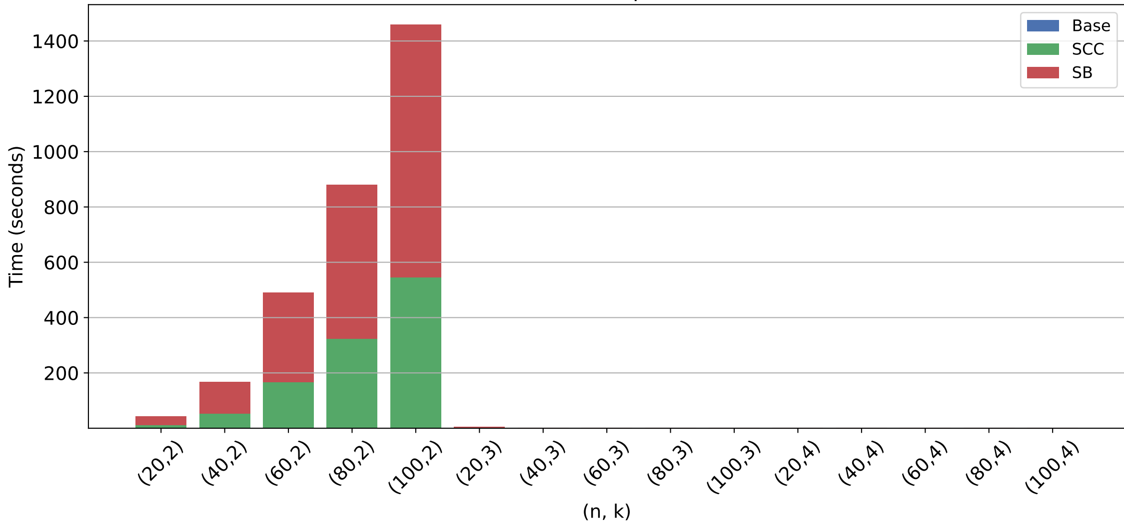
Time Breakdown per Instance
