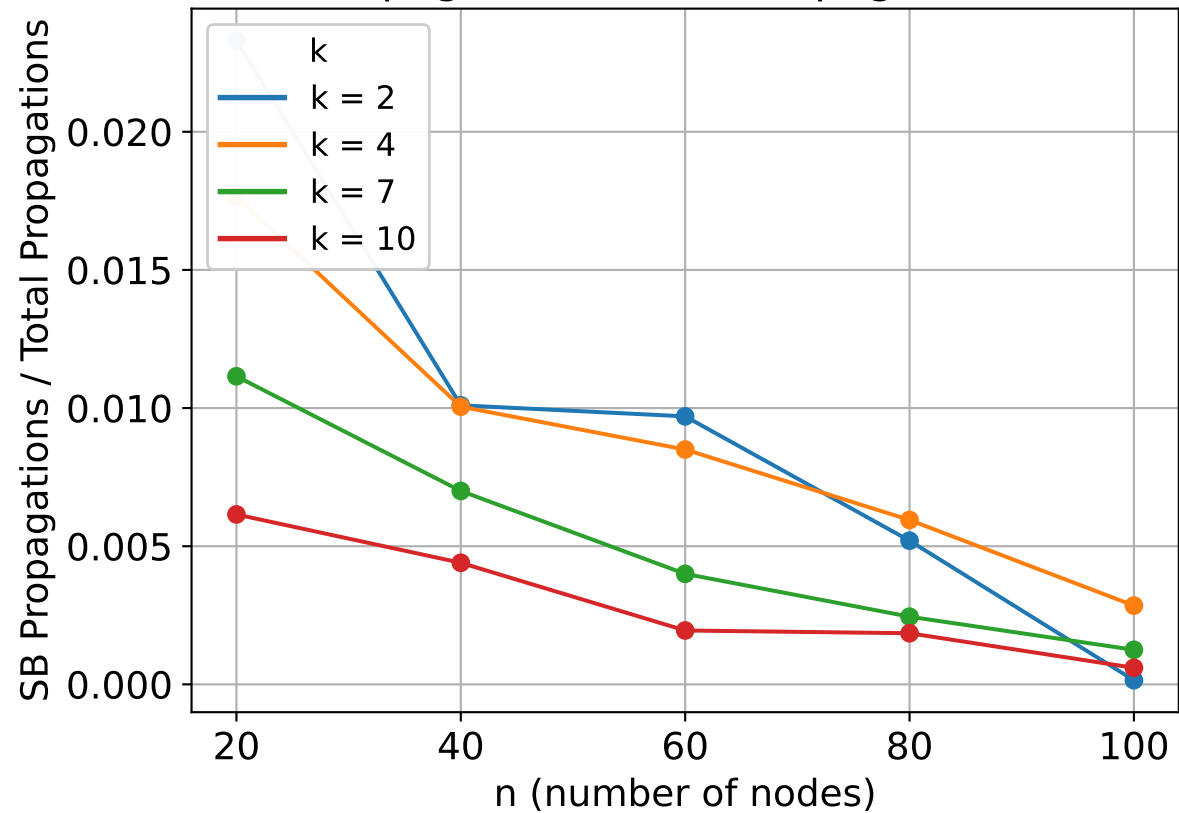
SB Propagations / Total Propagations vs n
