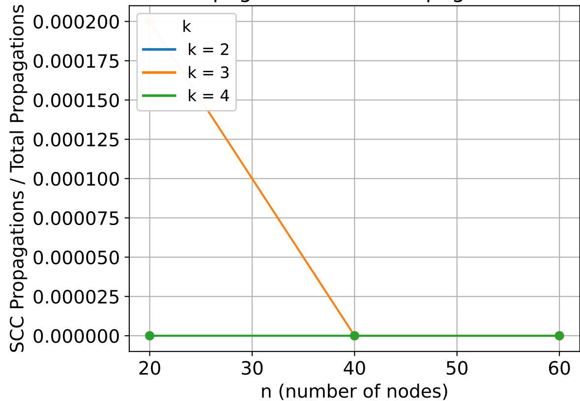
SCC Propagations / Total Propagations vs n
