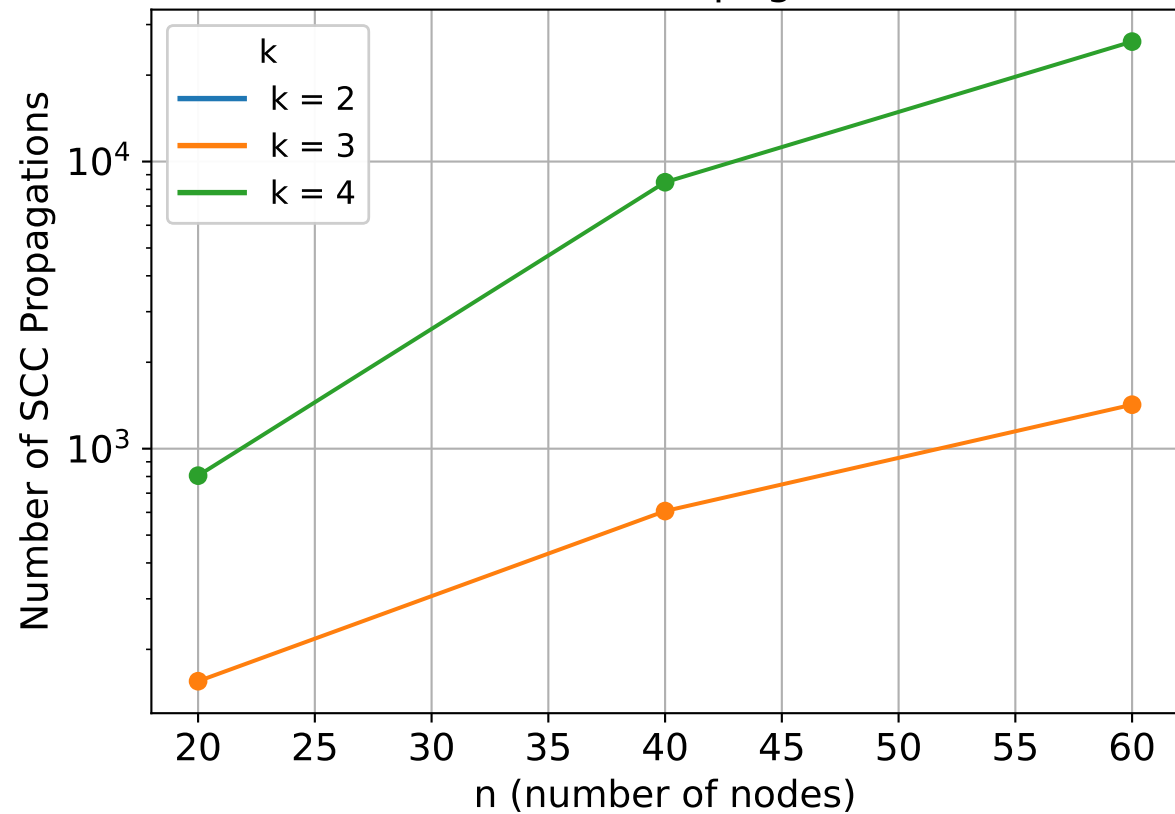
Number of SCC Propagations vs n
