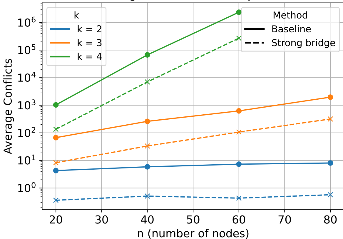
Average Conflicts vs Graph Size
