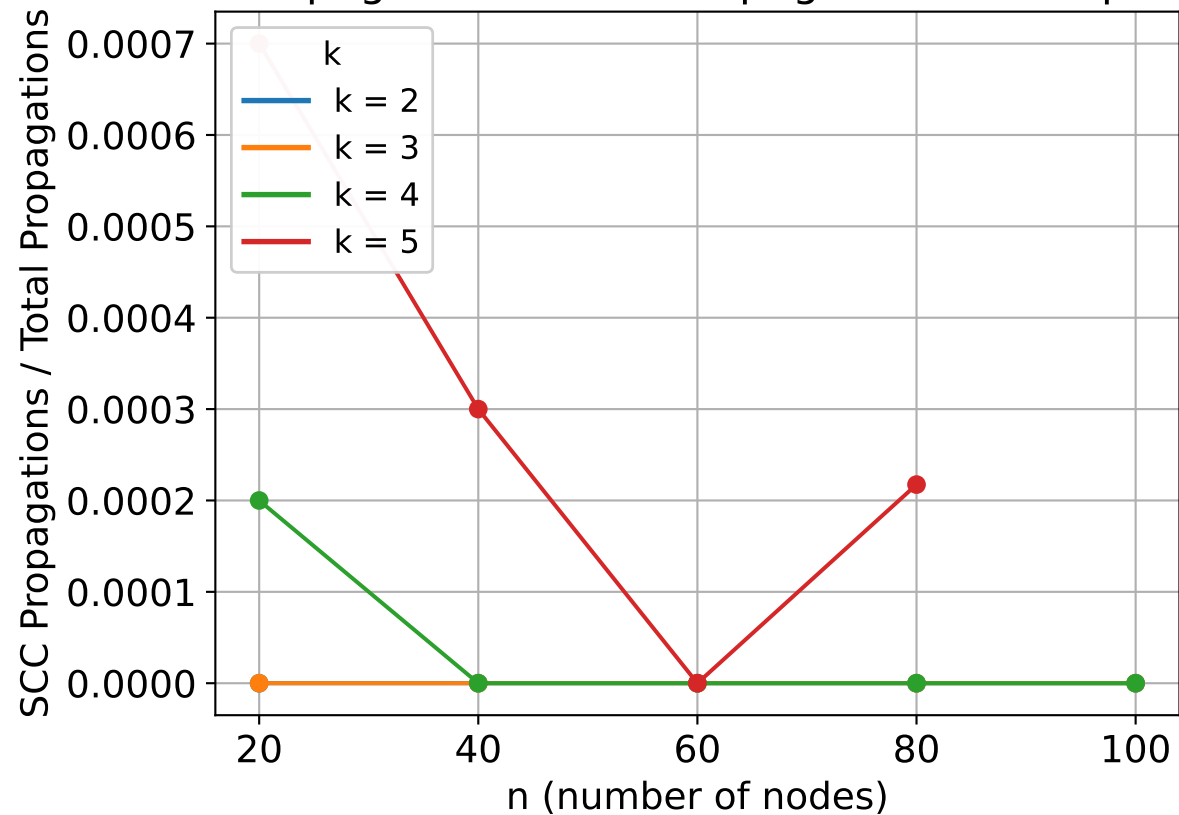
SCC Propagations / Total Propagations vs Graph Size
