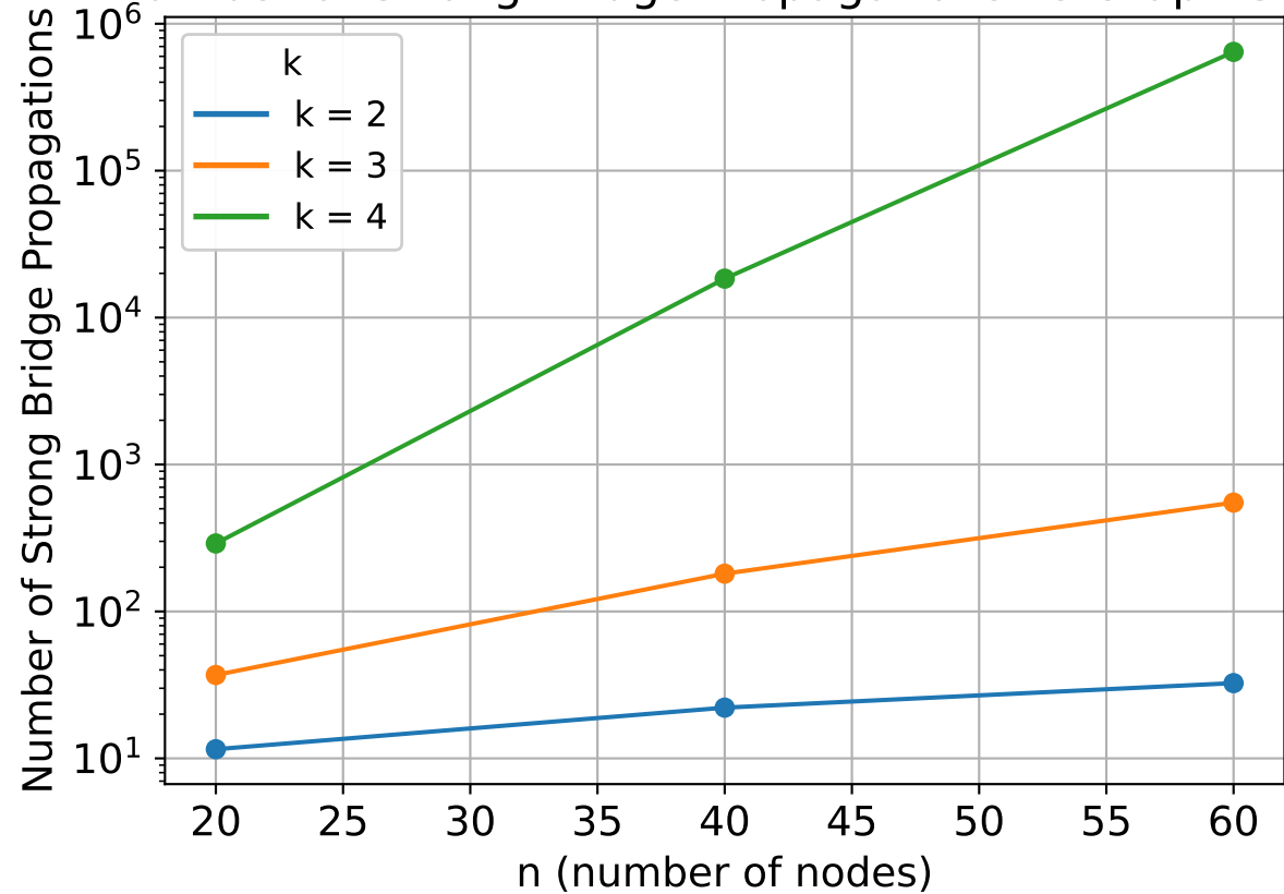
Number of Strong Bridge Propagations vs Graph Size
