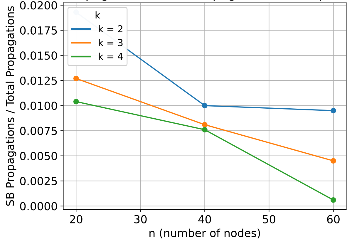
SB Propagations / Total Propagations vs Graph Size
