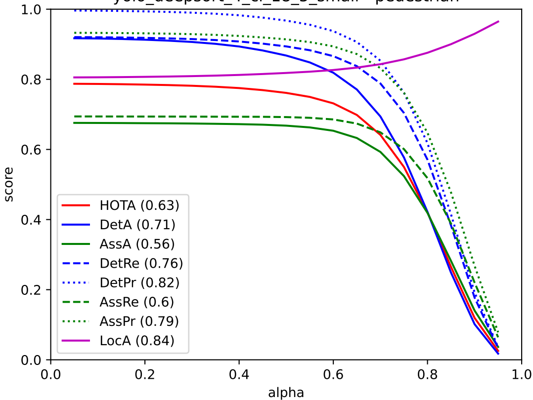
yolo_deepsort_4_cl_18_5_small - pedestrian
