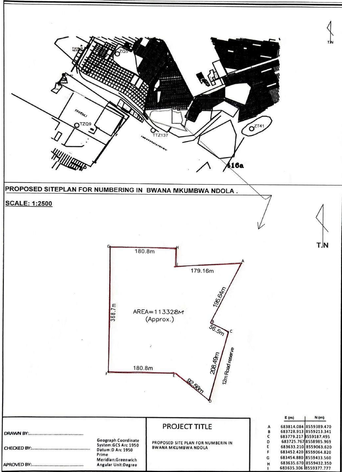
Figure 5: Site Plan showing the proposed numbering of a mining plot in Bwana Mkubwa
