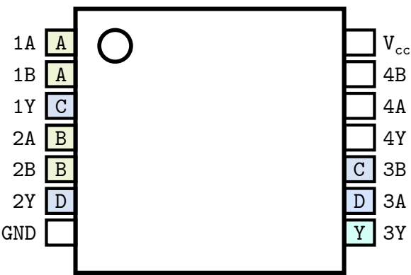
(b) Pin layout; and 2Y.
